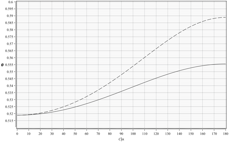
Fig. 4 The angular diameters of the luminaries (Sun: continuous curve , Moon: dash curve ) as a function of their anomalies ( C or \alpha ) based on Muh'yī al-Dīn's parameters
