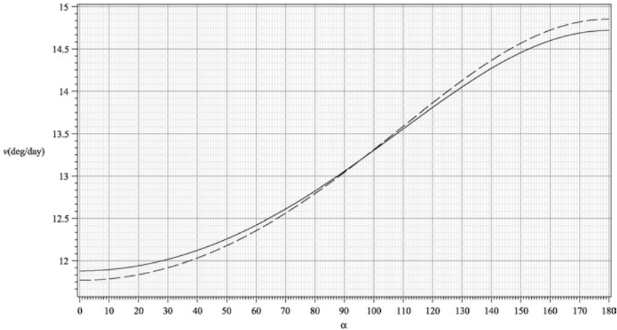
Fig. 3 The lunar instantaneous velocity according to the parameters of Ptolemy ( dash curve ) and Muh'yī al-Dīn ( continuous curve )
