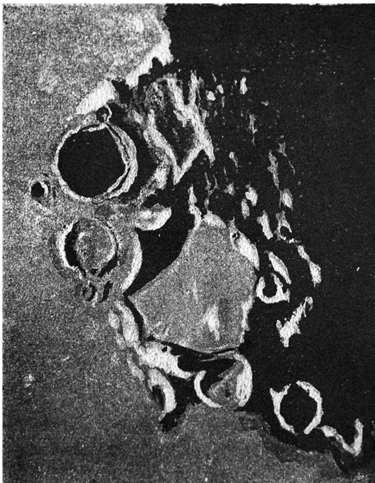
Fig. 6 Moraes Pereira drawing of the vicinity of the lunar crater Flammarion made on 2 July 1892 (Anonymous 1893b ; Flammarion 1893c )
