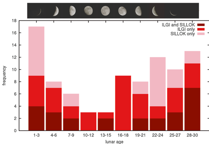
Fig. 3 Variation in the frequency with lunar age of sightings of “vapours like fire light” recorded in the Korean chronicles Seungjeongwon Ilgi ( Daily Records of the Royal Secretariat ) and Joseon Wangjo Sillok ( Veritable Records of the Joseon Dynasty ) between the beginning of 1625 and the middle of 1628. Note that the pattern in this figure is skewed, partly as a result of the excess of observations made in the early hours of the night
