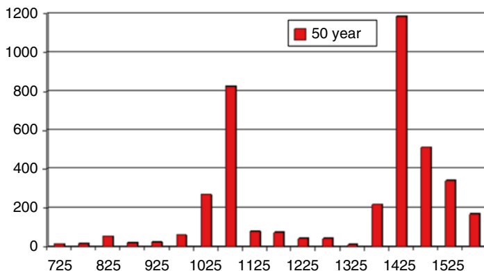
Fig. 1 Histogram showing the number of days on which meteors were recorded in 50 year intervals, from 701–1600 CE
