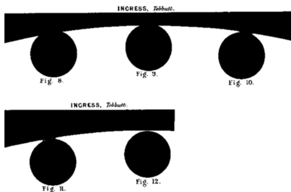
Fig. 54 Tebbutt's observations of the ingress of the 1874 transit of Venus (After Tebbutt 1883)
