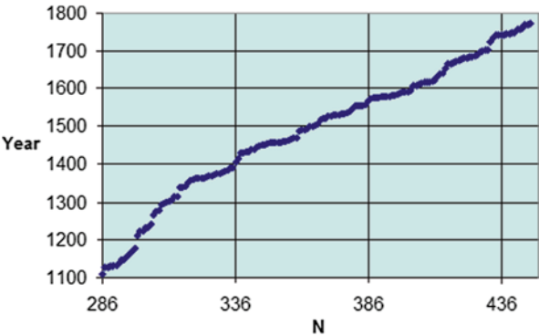
Fig. 4 Comets recorded in Chinese annals from 1100 to 1700. The format is the same as in Fig. 3
