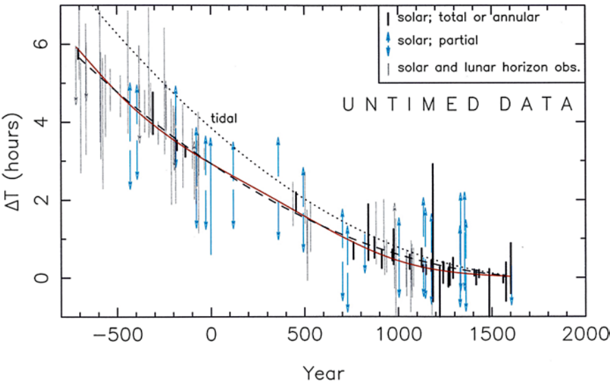
Fig. 4 The results for \Delta T derived from untimed eclipses. The dashed line is the best-fitting parabola, equivalent to a constant acceleration in the Earth's rotation. The red line is the best-fitting curve to all the data in Figs. 4 and 5. The varying slope of this curve denotes changes in rate of rotation on a timescale of millenia. The dotted parabola is the predicted change due to tidal friction
