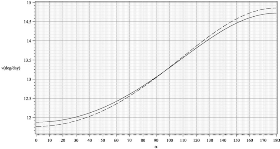
Fig. 3 The lunar instantaneous velocity according to the parameters of Ptolemy ( dash curve ) and Muḥyī al-Dīn ( continuous curve )
