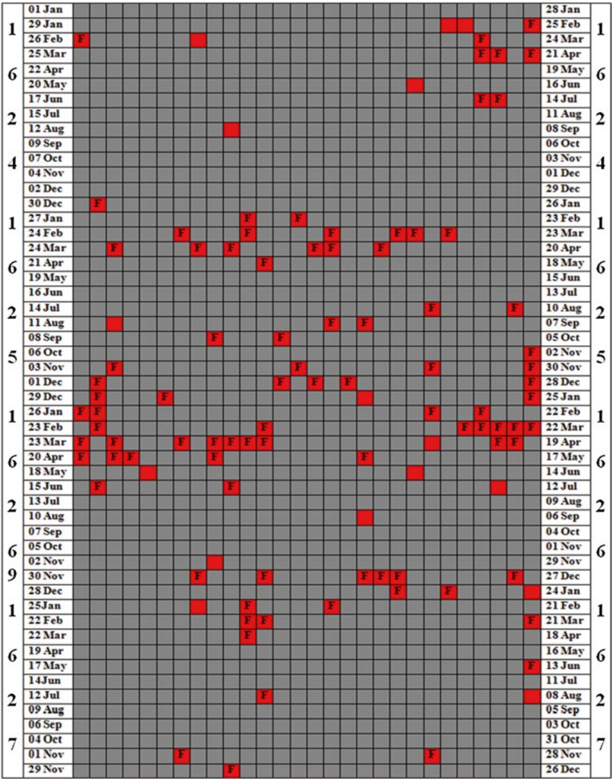
Fig. 6 The same as Fig. 5 but with all known auroral observations now coloured red, irrespective of the colour(s) quoted in the historical records. The letter ‘F’ is included to distinguish between an apparently featureless (F) red glow, which is described in the historical records as a “vapour like fire light”, and an auroral display exhibiting either structure or a colour other than red. All other qualifying letters (i.e. B and J) are omitted, as are the sunspot observations (●). Visual inspection of Fig. 6, or Fig. 5, reveals two examples of a (vertical) sequence of four auroral observations separated by exactly 28 days. Further visual inspection of either figure reveals one example of auroral observations on six consecutive nights and one example of auroral observations on four consecutive nights. The statistical significance of the pattern of auroral events shown in Fig. 6 is discussed in Sect. 7
