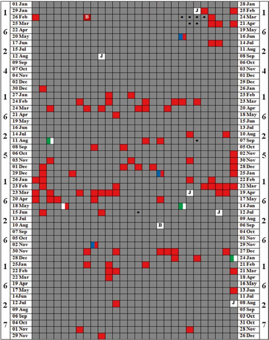
Fig. 5 Similar to Fig. 4 but with all known auroral observations in the interval 1 January 1624–26 December 1627 included. This figure shows the correct colour(s) of the auroral observations, as recorded in the appropriate East Asian history. If compound colours are quoted, both colours are shown. The letter ‘B’ signifies that the corresponding Korean auroral observation was recorded in the Jeungbo Munheon Bigo : the observation on the evening of 4 March 1624, which is described as being “dark”, is provisionally represented by the colour “dark red”. The letter ‘J’ signifies that the corresponding Japanese auroral observation was found in the catalogue published by Osaki (1994): the colour of these Japanese observations is tentatively assumed to be “white”. Solid dots (●) signify the days on which sunspots were observed in East Asia (although the background colour of each small square refers solely to night-time conditions)
