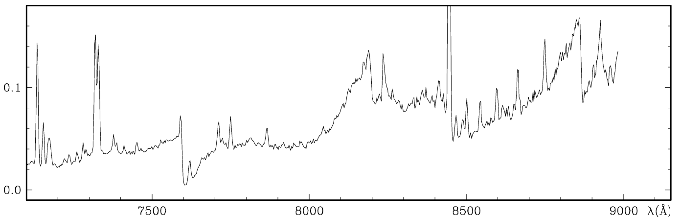
Fig. 86. ESO 1.5m + B&C spectrum of V1016 Cyg
