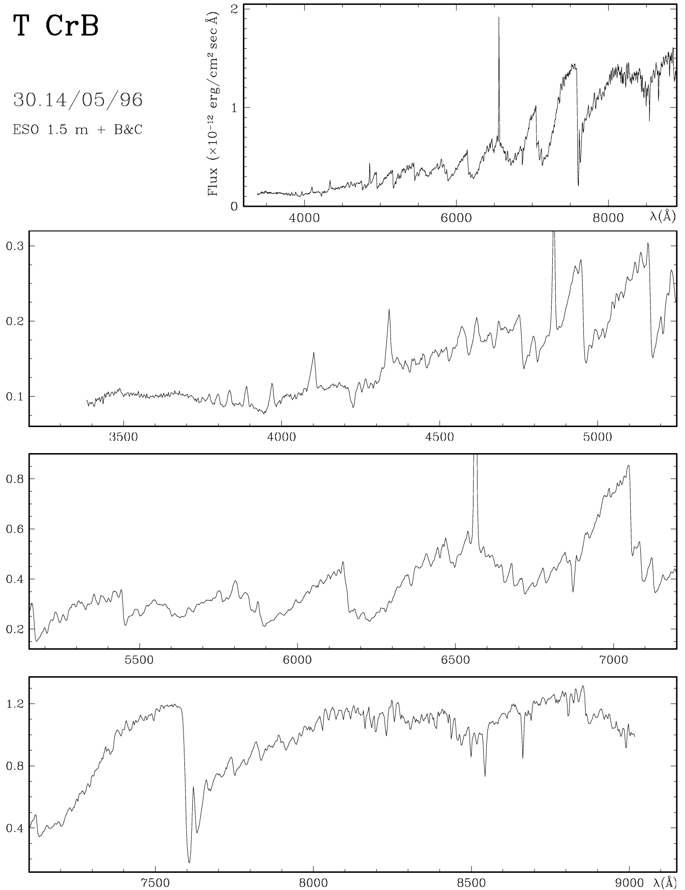
Fig. 41. ESO 1.5 m + B&C spectrum of T CrB
